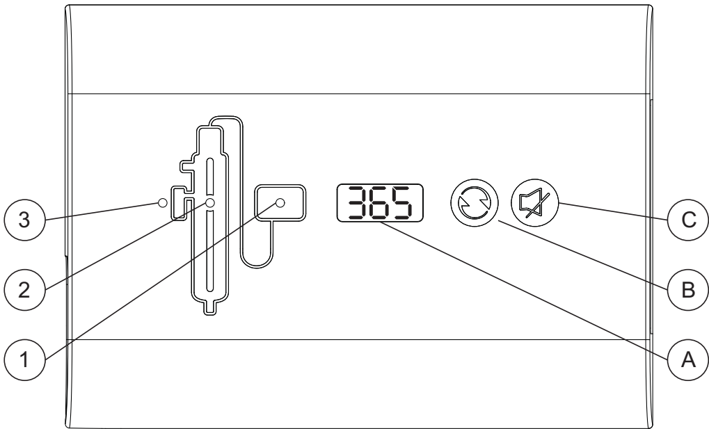
Figure 4 Control Panel
